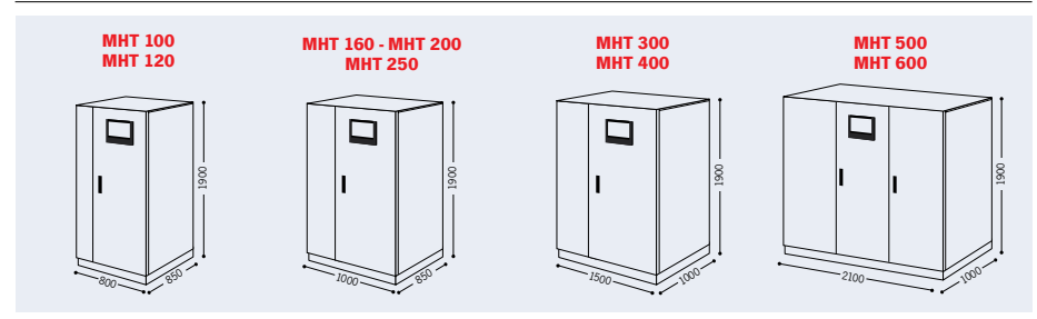
dimensions (mm)
